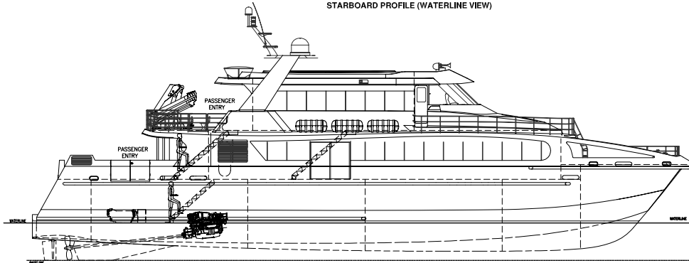
STARBOARD PROFILE
