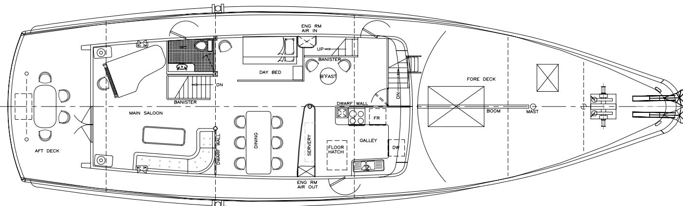
PLAN MAIN DECK
