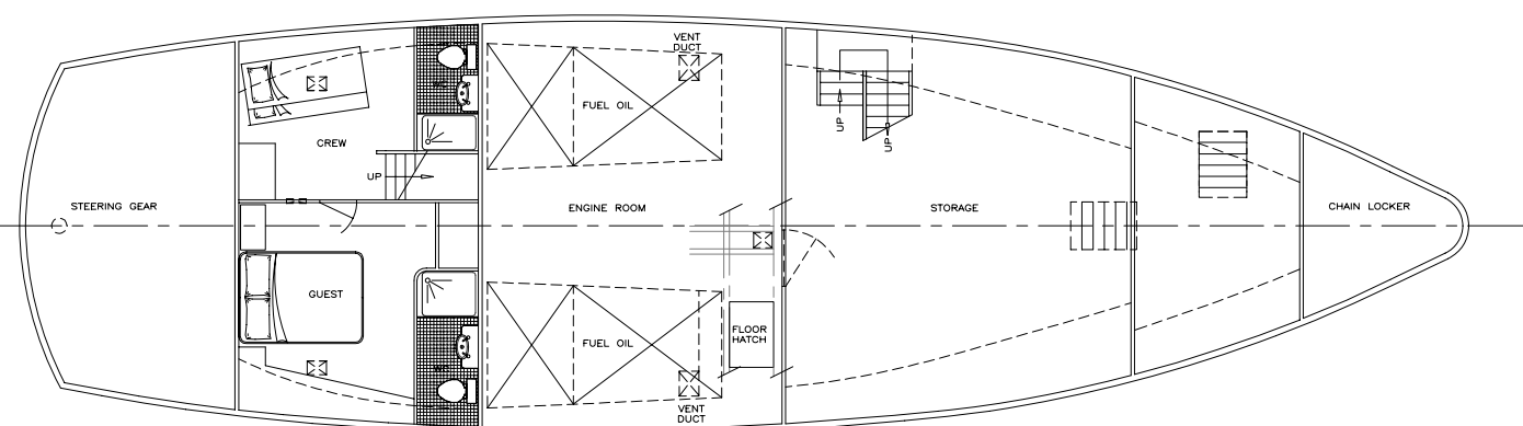
PLAN LOWER DECK
