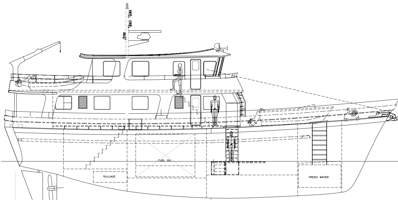
CENTRELINE PROFILE
