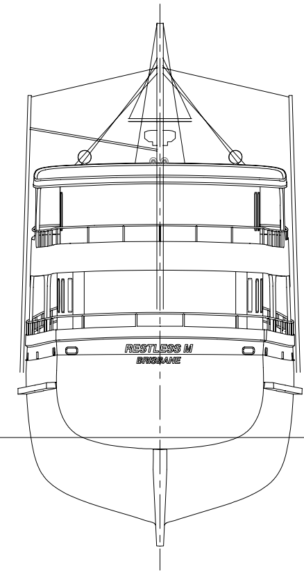
STERN VIEW LOOKING FWD
