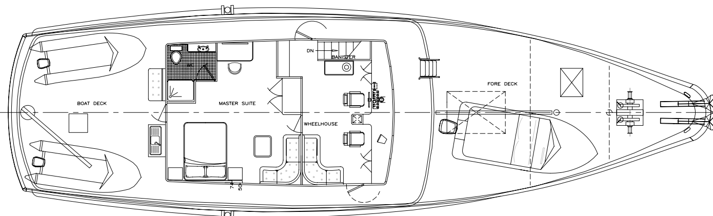
PLAN UPPER DECK
